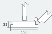
MFC/HPL Pilaster Section
