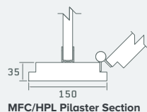
MFC/HPL Pilaster Section
