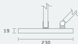
MFC/HPL Pilaster Section
