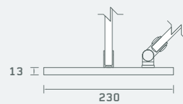
SGL Pilaster Section
