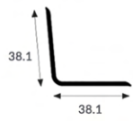
1.5° INTERNAL ANGLE *
