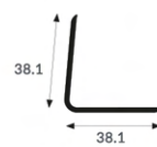
1.5° EXTERNAL ANGLE *
